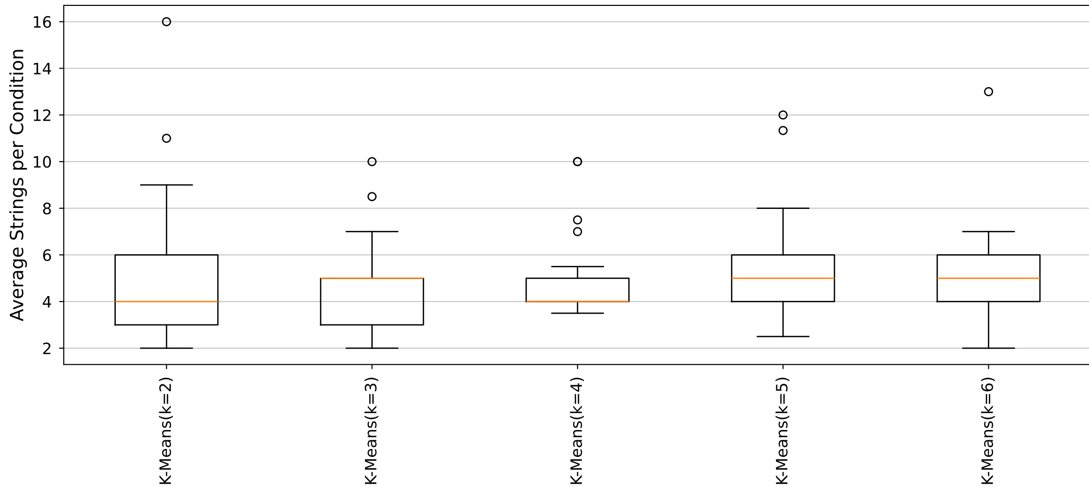
YARA Rules Average Strings per Condition Distribution (Cluster27_Size6 dataset)
